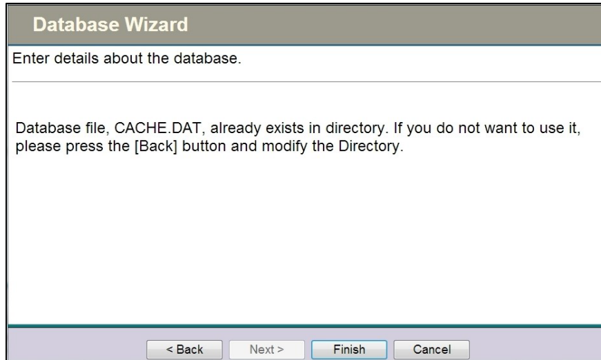
Figure 4-10: Database Wizard
