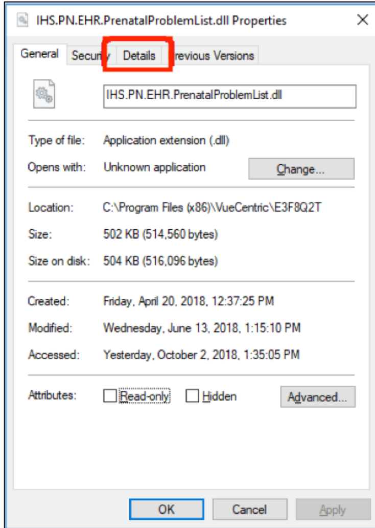
Figure 2-5: Properties window
