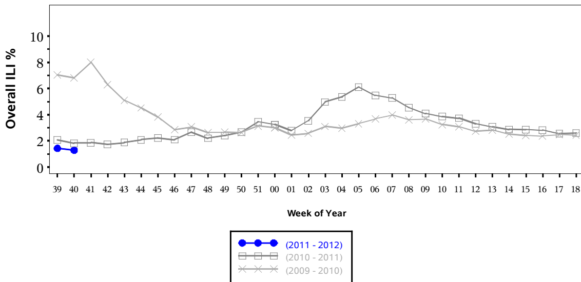
Percentage of Visits for Influenza-like Illness (ILI) per week Overall ILI % (ILI visits per week / Total visits per week) (ILI) in IHS, October through April
