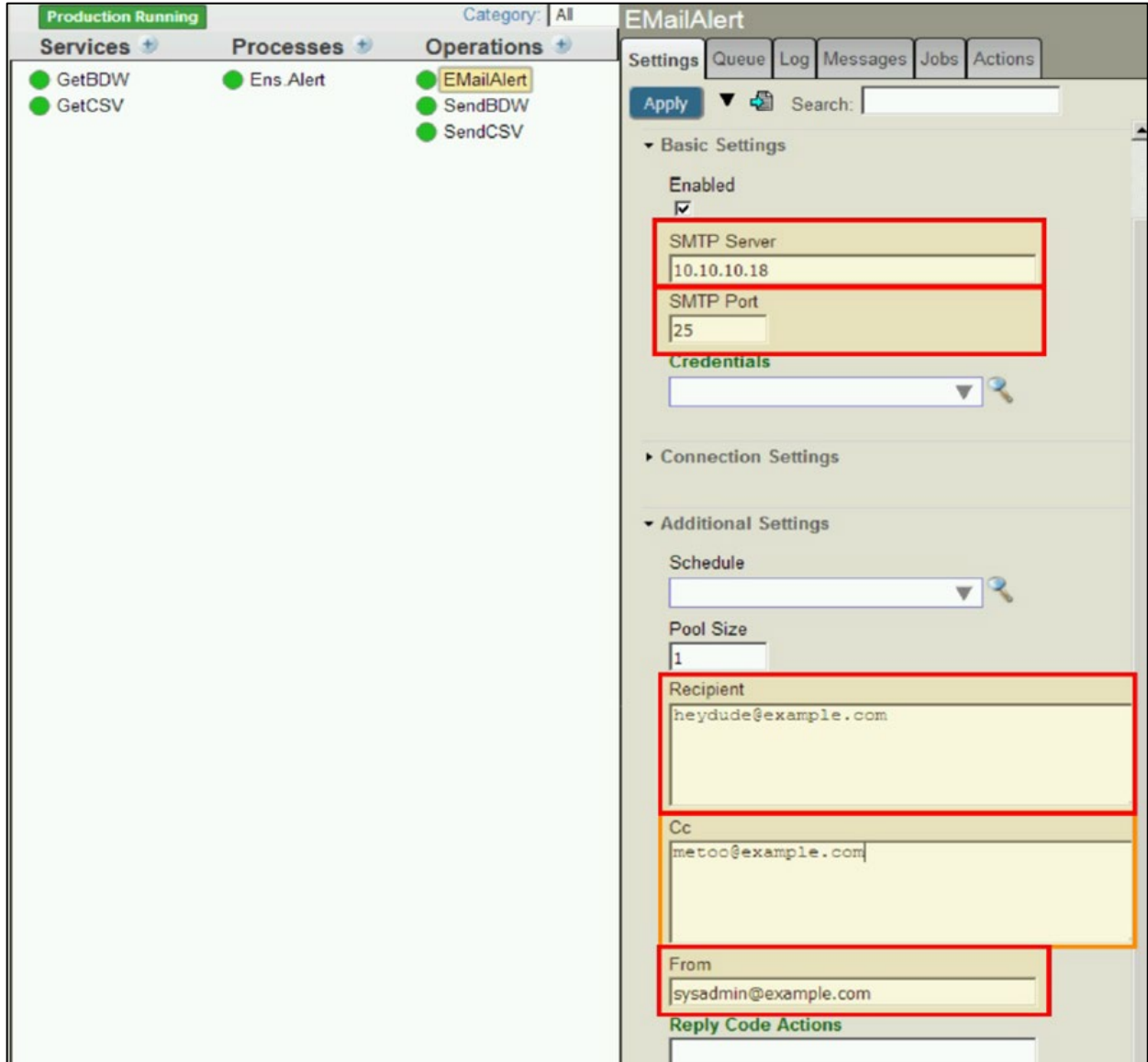
Figure 3-8: Email settings
