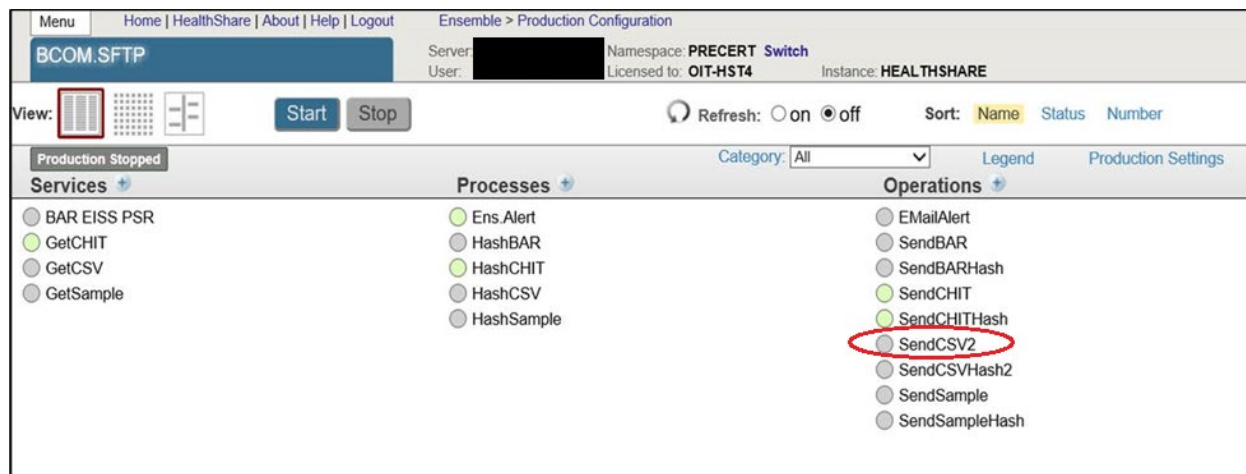
Figure 3-7: Send CSV2 operations
