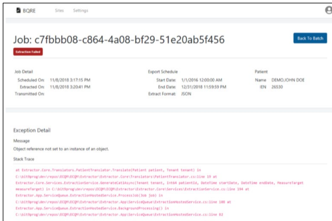
Figure 2-20: Failed reason detail window
