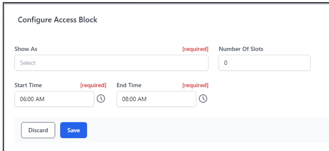
Figure 3-23: Configure Access Block dialog
