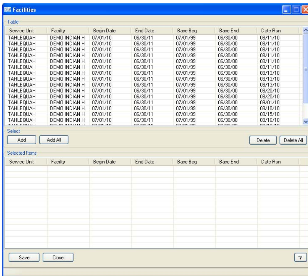
Figure 5-4: Facilities window
