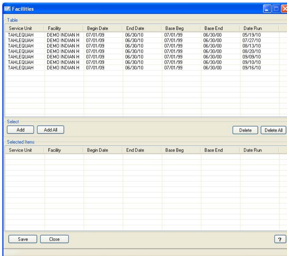
Figure 5-22: Facilities window
