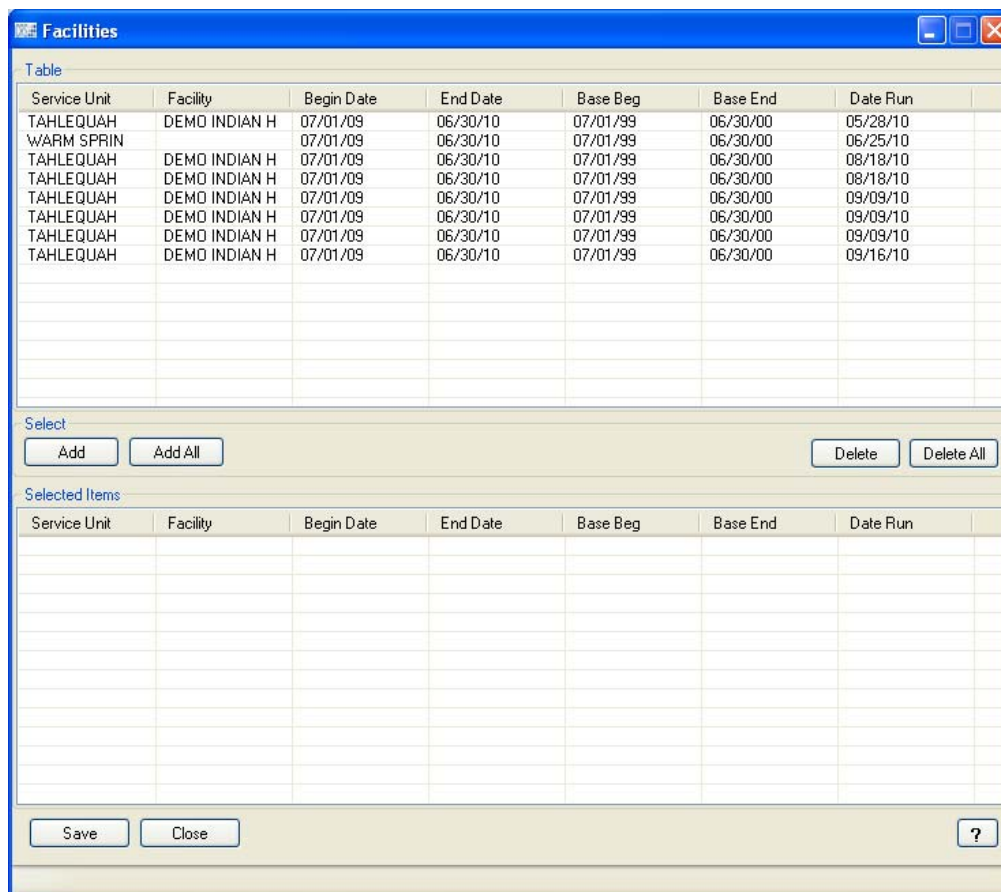
Figure 5-10: Facilities window
