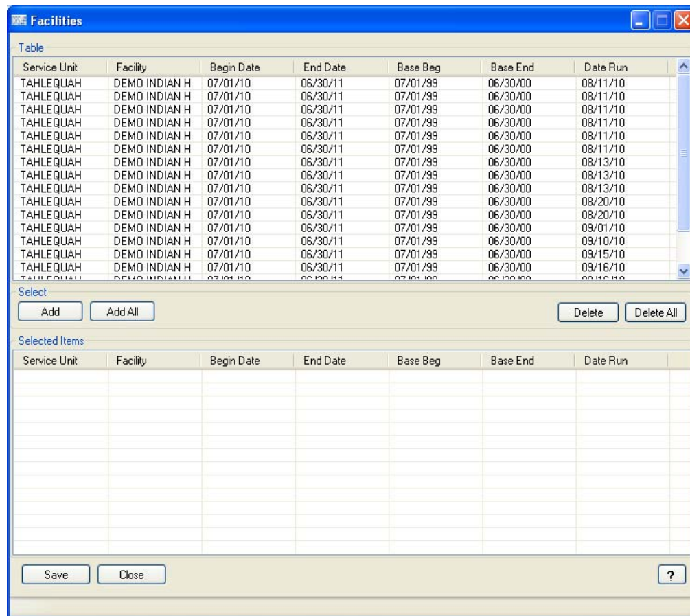
Figure 5-8: Facilities window
