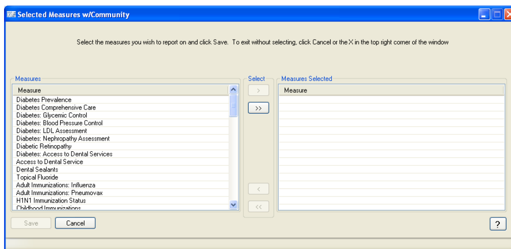
Figure 6-33: Measures window
