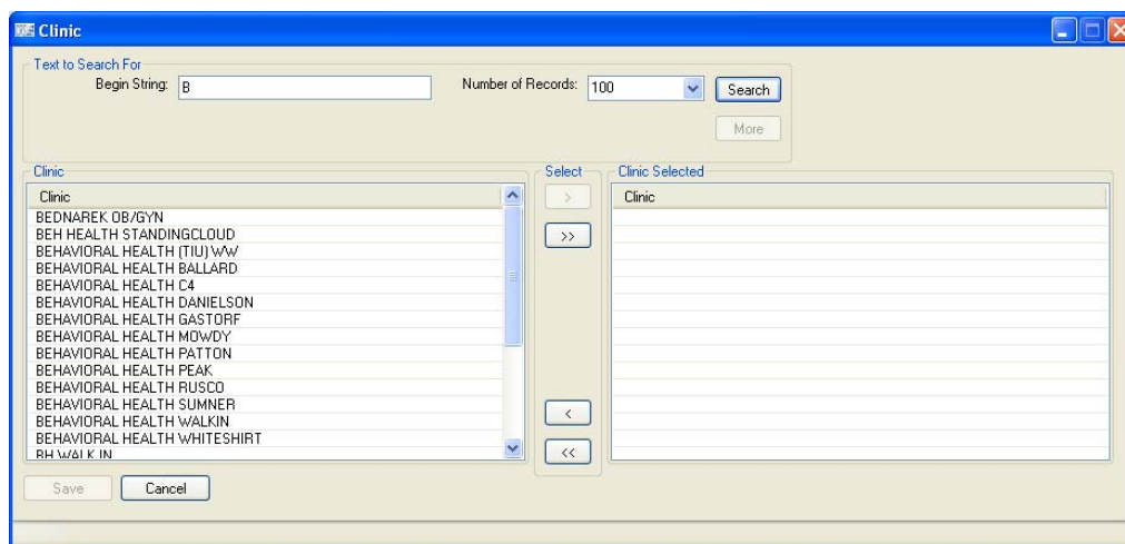
Figure 6-18: Clinic window
