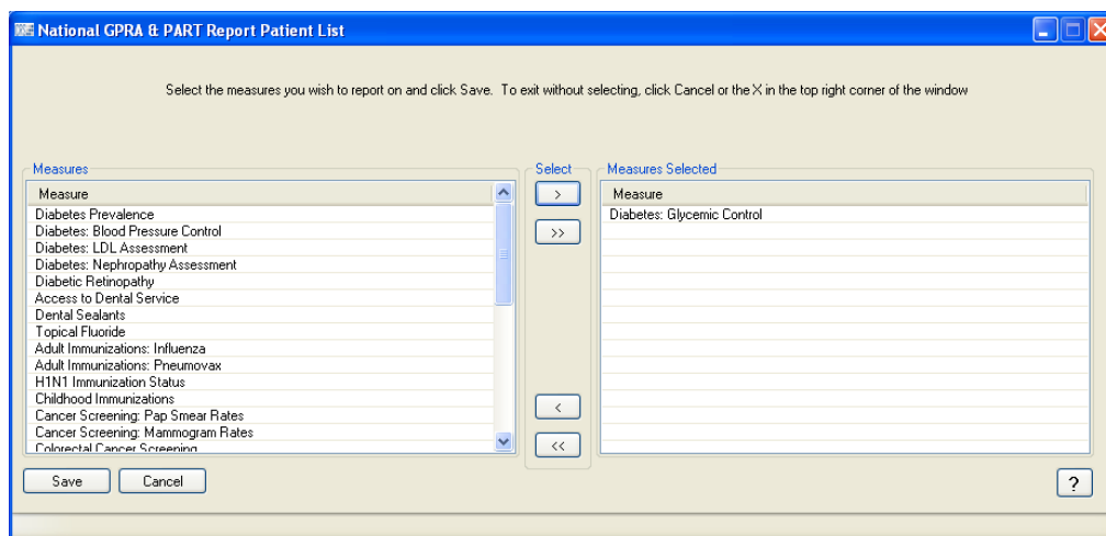
Figure 6-21: Measures window
