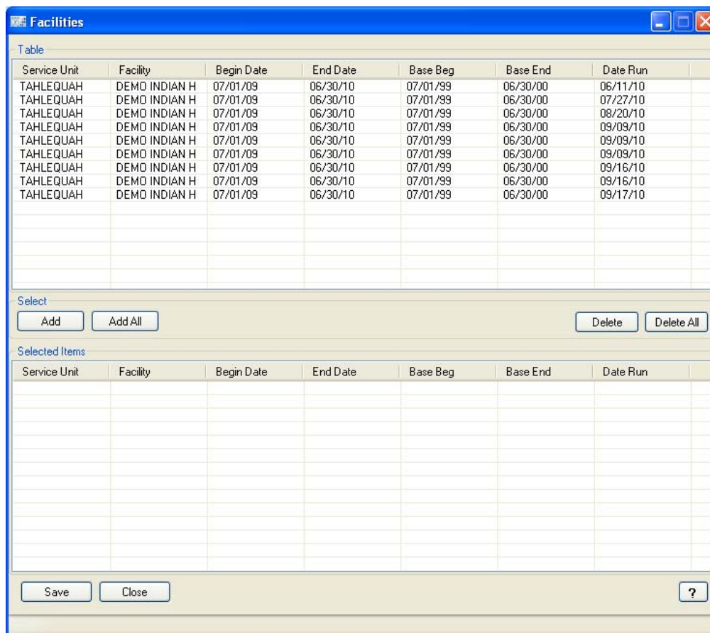
Figure 5-15: Facilities window
