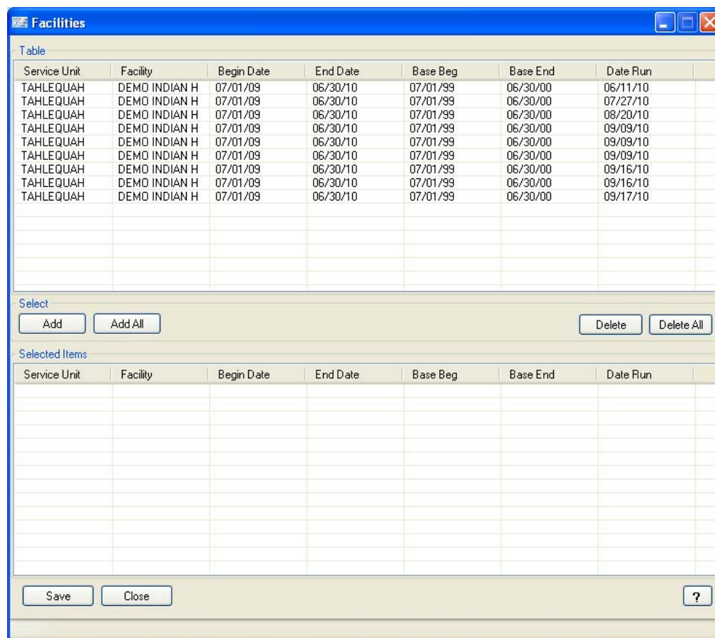
Figure 5-13: Facilities window
