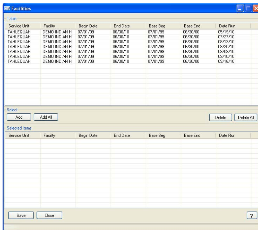
Figure 5-18: Facilities window
