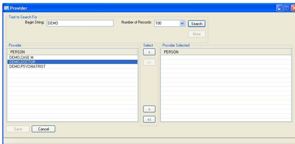
Figure 6-12: Provider window
