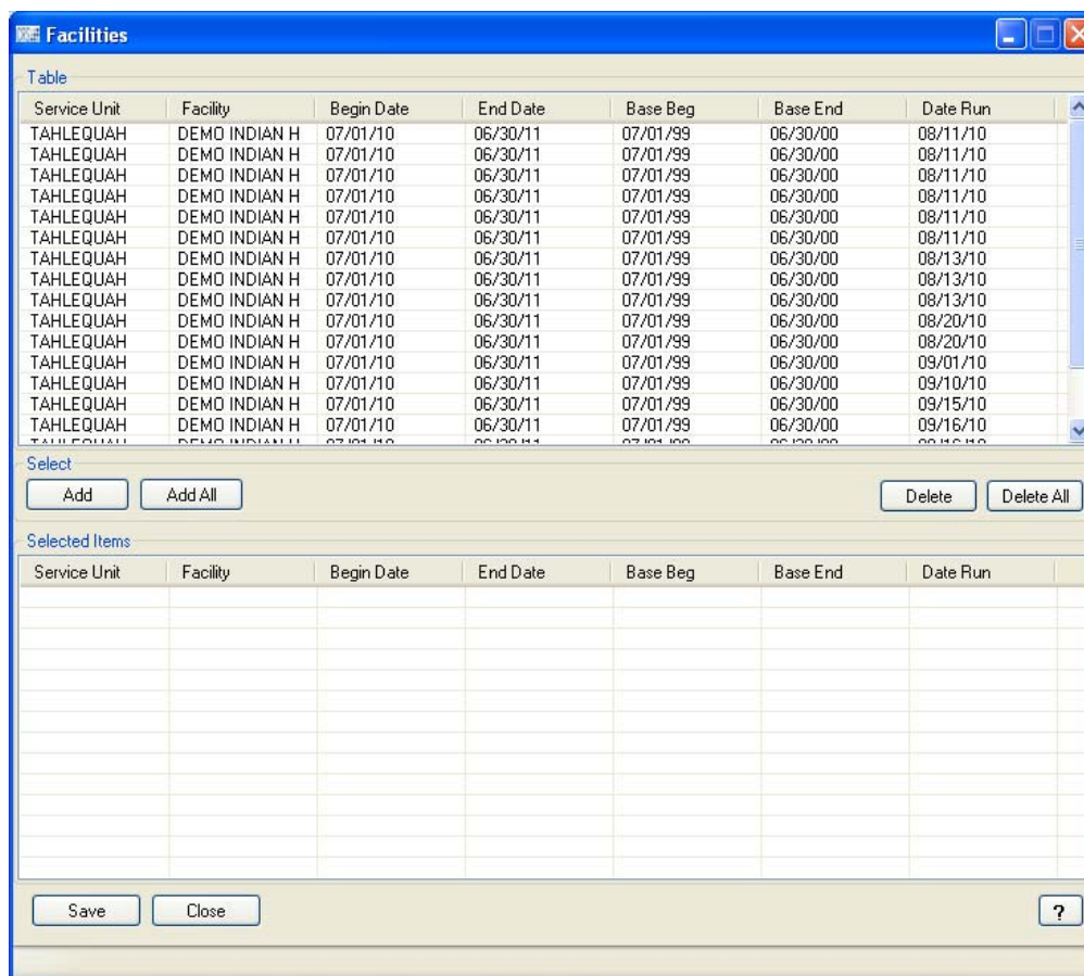
Figure 5-6: Facilities window
