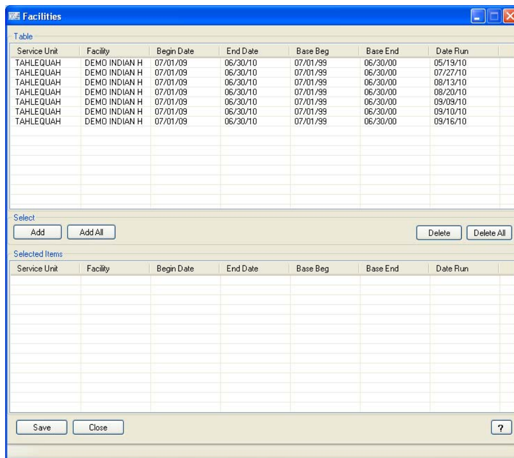
Figure 5-28: Facilities window
