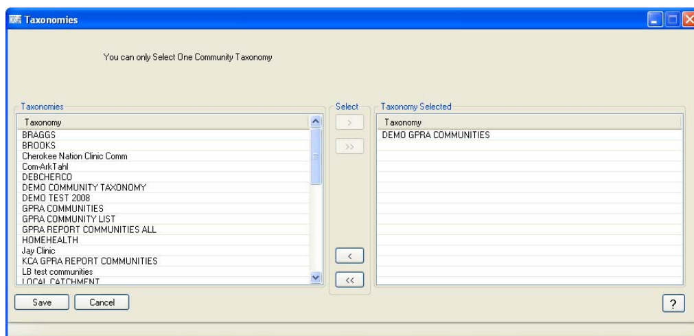
Figure 6-6: Taxonomies window
