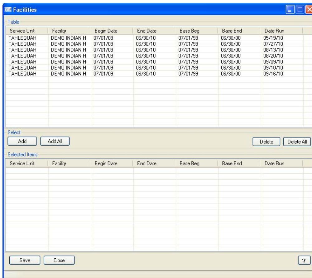
Figure 5-20: Facilities window
