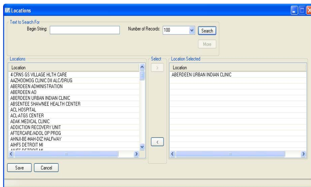
Figure 6-10: Locations window
