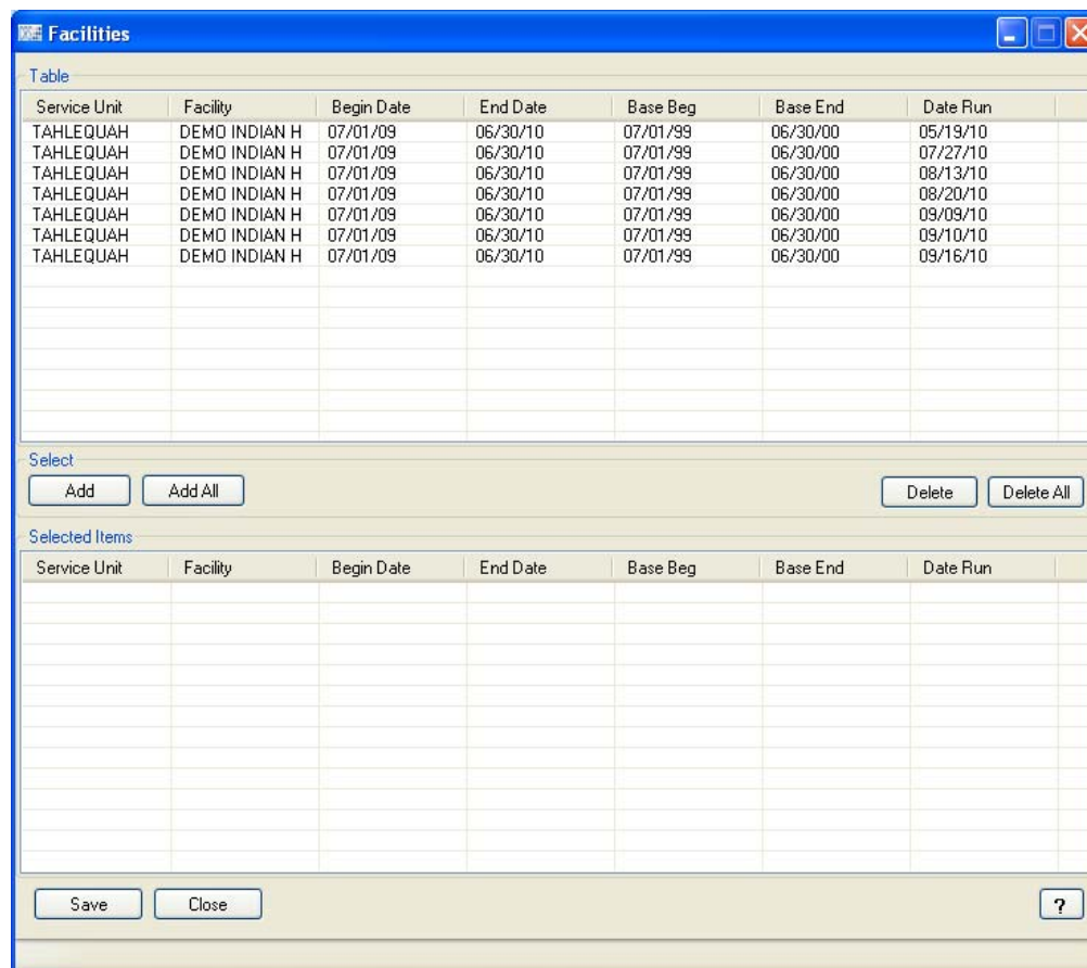
Figure 5-26: Facilities window
