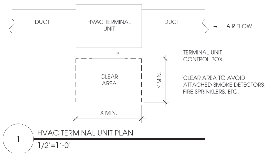
Figure 1. HVAC Terminal Units
